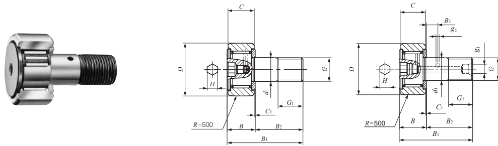
CF...BR Zapfendurchm. d_1 3-10mm
