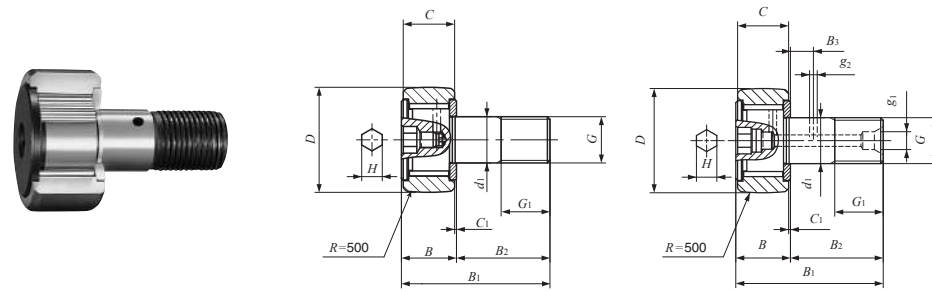
CF...VBR Zapfendurchm. d_1 6-10mm
