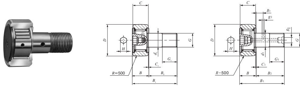
CF...WBR Zapfendurchm. d_1 3-10mm
