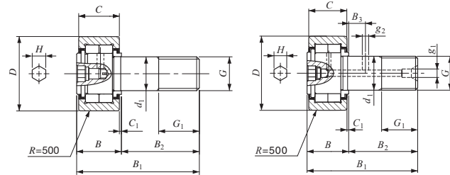
NUCF...BR Zapfendurchm. d_1 10mm
