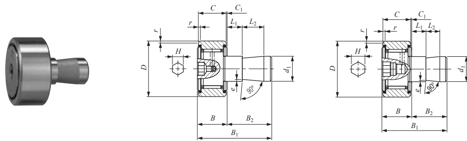
CF-SFU...B Zapfendurchm. d_1 6-10mm
